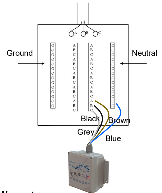
The Satic Power Perfect Box should be placed on a dedicated, 3-pole 50 amp breaker (not included).
