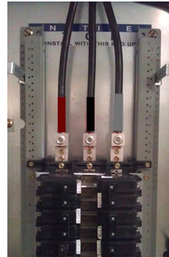
The Satic Power Perfect Box should be placed on a dedicated, 3-pole 50 amp breaker (not included).
